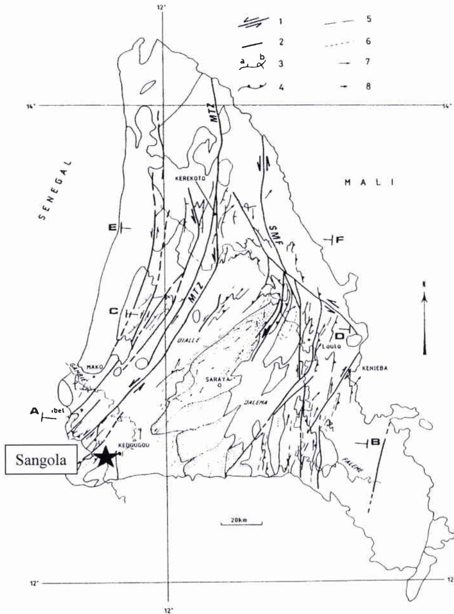
Structural map of the Kedougou inlier, Senegal and Mali: 1 = transcurrent fault; 2 = reverse fault; 3 = trace of stratification in B2 (a = normal position, b = reverse position); 4 = trace of schistosity 1 in B1; 5 = trace of schistosity 2; 6 = planar fabric in the granites; 7 = stretching lineation; 8 = linear fabric in the granites; MTZ = Main Transcurrent Zone; SMF = Senegalese-Malian Fault.
